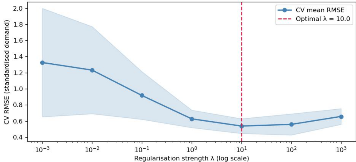
Ridge — 5-fold TimeSeriesSplit CV
