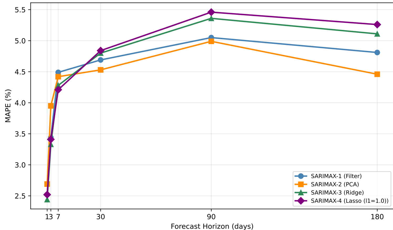
SARIMAX Variants — MAPE vs Forecast Horizon (Test Set)
