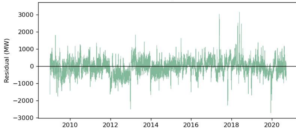
SARIMAX-3 (Ridge) std=493 MW, R^2=0.849
