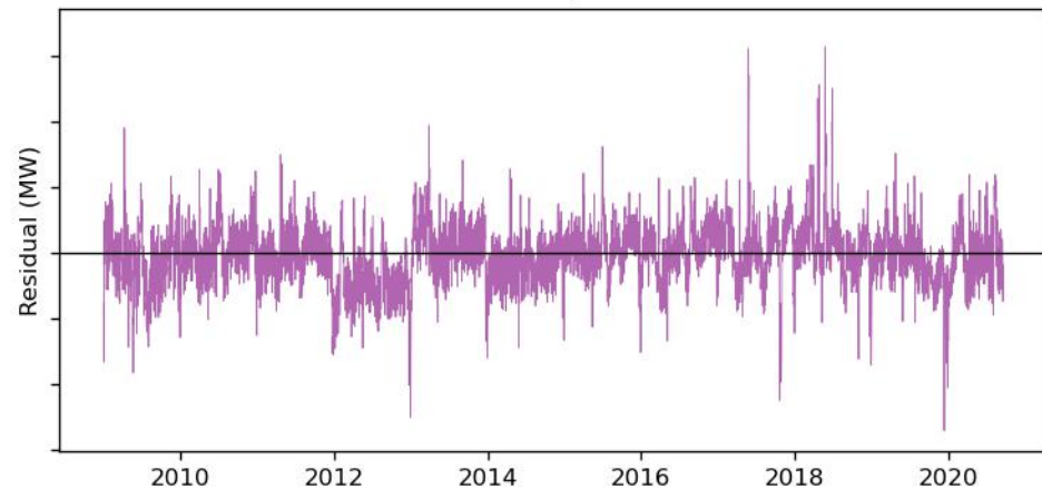
SARIMAX-4 (ElasticNet) std=493 MW, R^2=0.849
