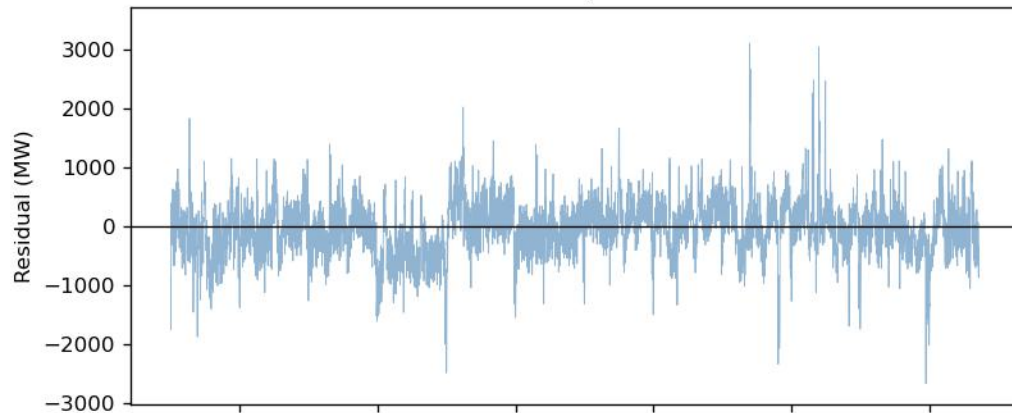
SARIMAX-3 (Ridge) std=493 MW, R^2=0.849
