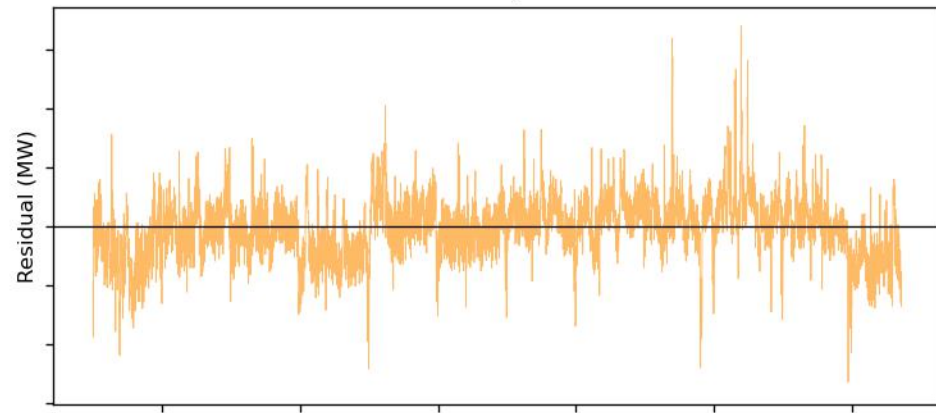
SARIMAX-4 (ElasticNet) std=493 MW, R^2=0.849
