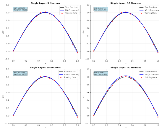
Approximation quality vs network width
