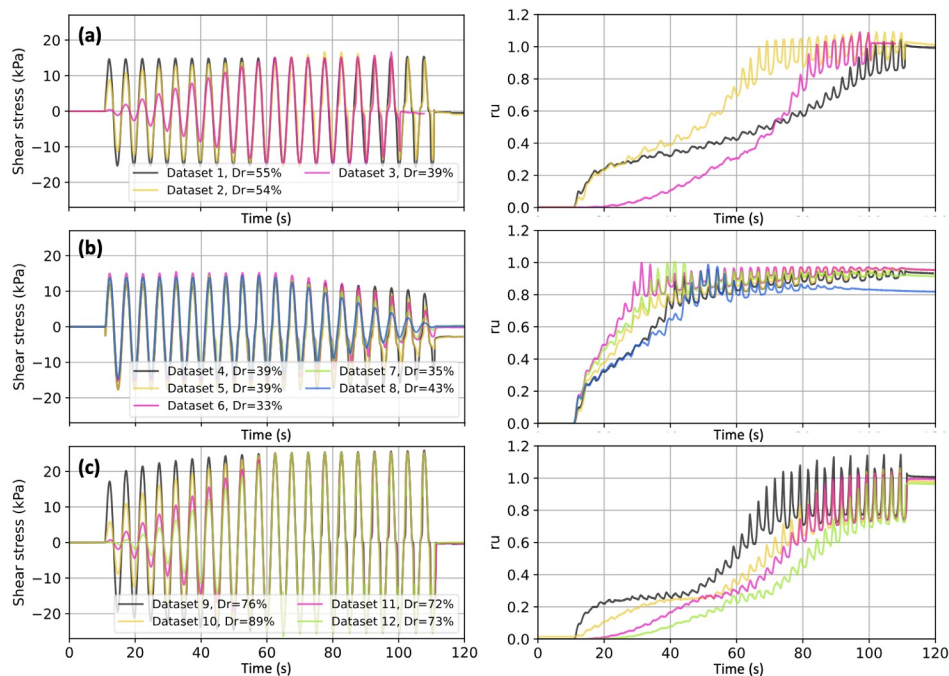
Figure 3. The responses of pore water pressure ( r_u ) corresponding to different input shear stresses and sample relative densities ( D_r ) for 12 laboratory cyclic simple shear tests (Kwan et al., 2017): (a) one harmonic and two modulated-up stresses on loose samples; (b) five modulated-down stresses on loose samples; (c) four modulated-up stresses on dense samples.
