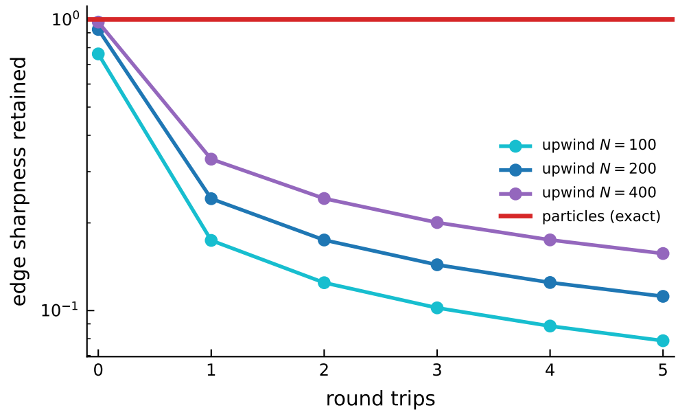
(b) Numerical diffusion flattens the front at every resolution
