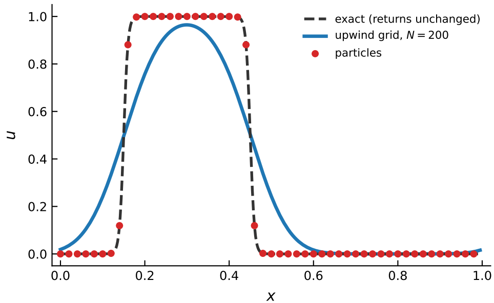
(a) The front after 5 round trips
