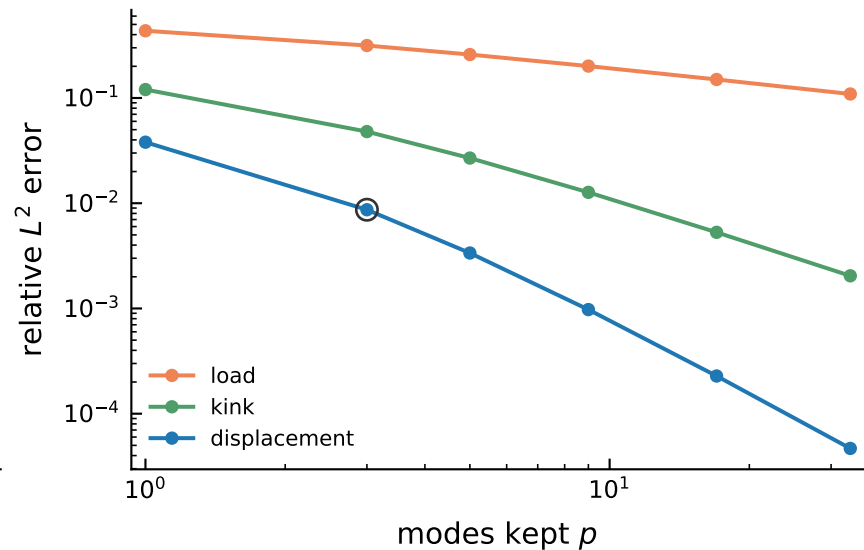
truncation error
