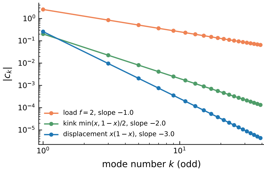
coefficient decay
