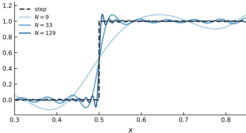
sine partial sums of a step
