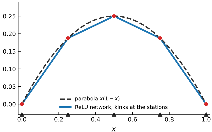
largest gap 0.0156, bound Mh^2/8 = 0.0156
