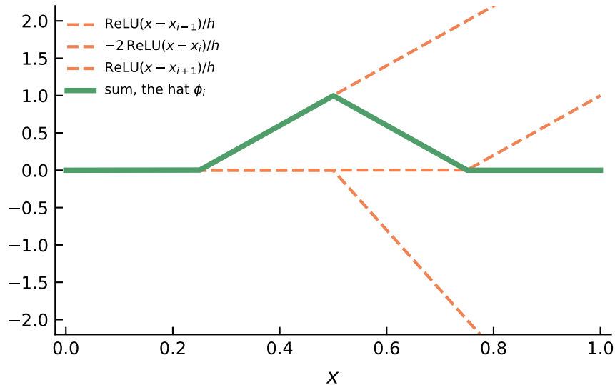
one hat from three ramps ( h = 0.25 )
