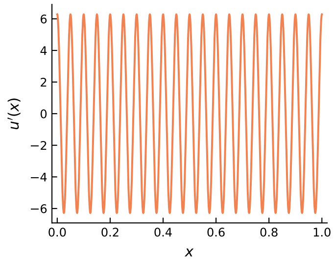
wiggle slope: |\cdot|_{H^1} = 4.44
