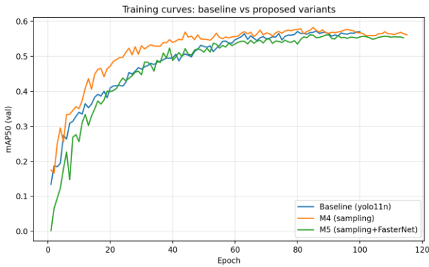
Fig. 3 Validation mAP50 over training. The sampled variant (M4) leads from early epochs; the combined variant (M5) tracks the baseline closely. Early stopping (patience 30) catches the mild over-fitting of M4 after its peak
