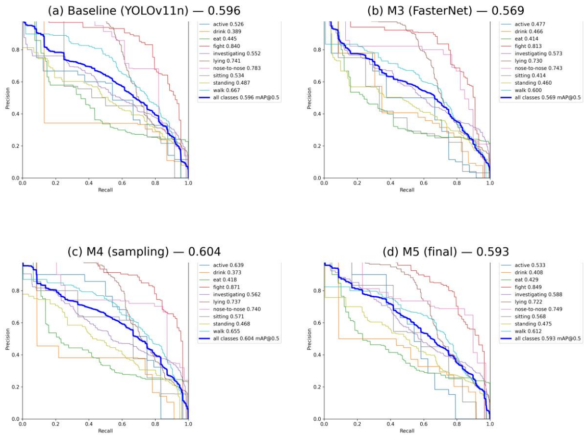
Fig. S1 Precision-recall curves on the held-out test set for the four ablation models: (a) baseline YOLOv11n (mAP50 0.596), (b) M3 FasterNet-only (0.569), (c) M4 sampling-only (0.604), (d) final M5 (0.593). Behaviour-class curves are shown thin; the thick blue curve is the all-class average
