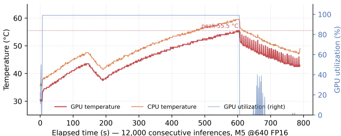
Fig. S3 Sustained-operation timeline on the Jetson Nano over 12,000 consecutive inferences (10.7 min, M5 at 640×640 FP16). Throughput holds at 20.0 FPS (99th-percentile latency 51.3 ms); GPU temperature peaks at 55.5 °C with zero thermal-throttling events and no clock drop
