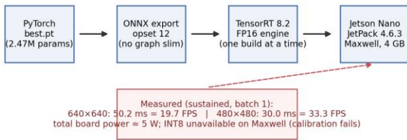
Fig. 7 Deployment pipeline from the PyTorch checkpoint to on-device TensorRT inference, with measured on-device performance and the practical constraints encountered
