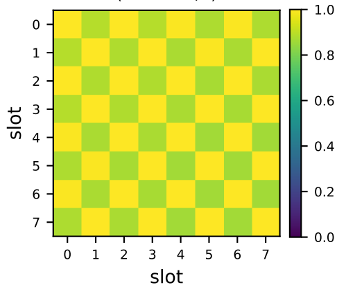
A — end-of-conv. bank (s42) slot cosine; eff. rank 1.13/8 (s43: 1.48/8)
