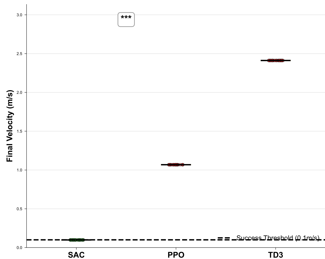
B Final Velocity Distribution
