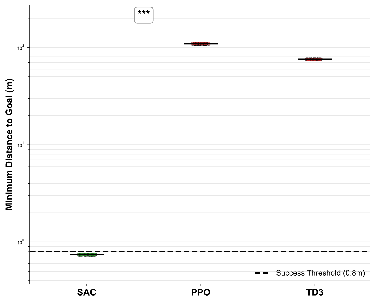
A Minimum Distance Distribution (Log Scale)
