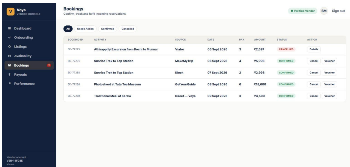
Figure 5. Fresh booking list and voucher action captured from the running Chrome application on 06 September 2026.
