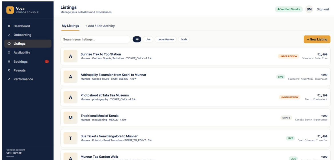
Figure 3. Fresh vendor Listings workspace captured from the running Chrome application on 06 September 2026. The Add or Edit Activity entry point is available in the same screen.
