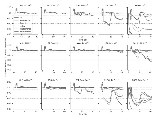
Figure 4 Predicted control-normalized response of population density over time, if all or only one toxicity component is simulated. In the model, effects on reproduction efficiency caused most of the effect across metals at low and intermediate effect concentrations. Responses above one (dashed line) are shown on a log-scale. Dotted lines indicate the 10% and 50% effect levels, respectively.
