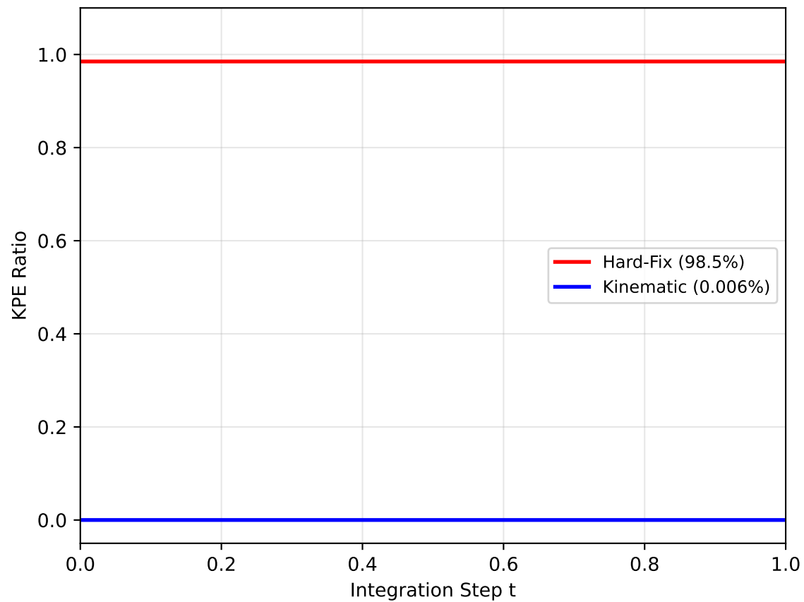
(c) Cumulative KPE Ratio
