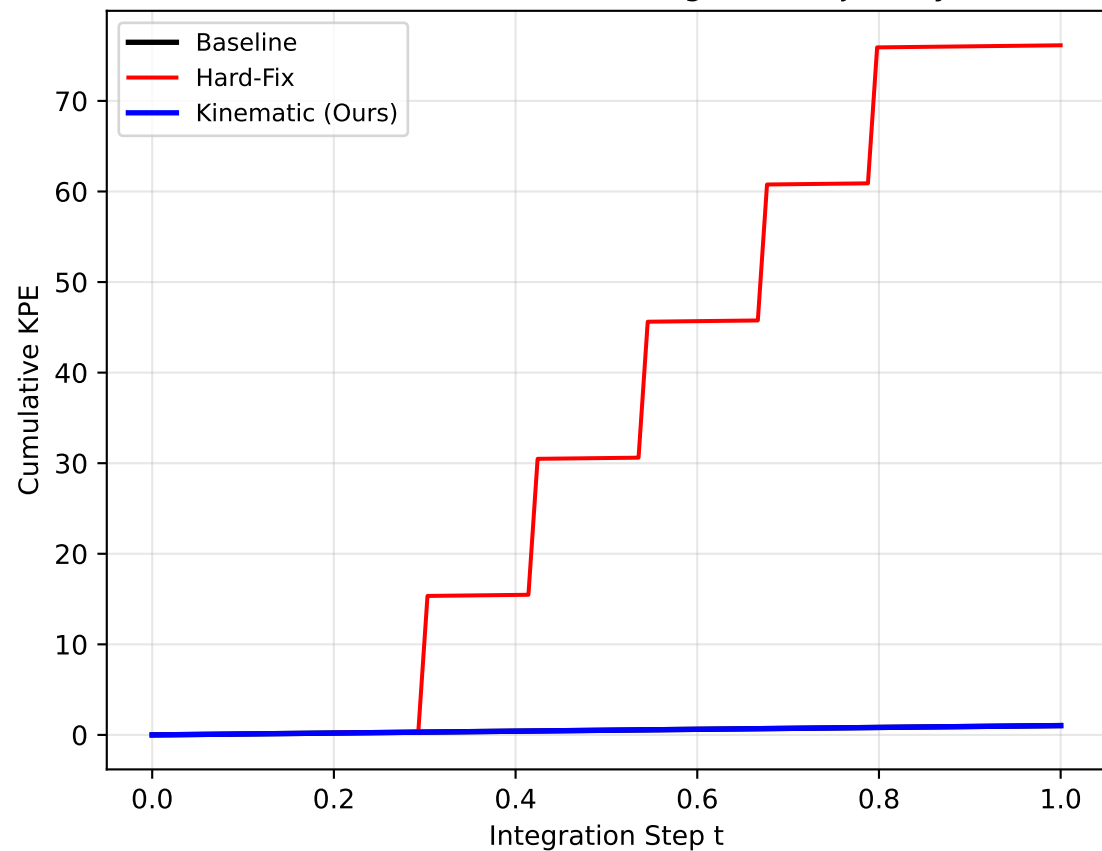
(c) Cumulative KPE Ratio
