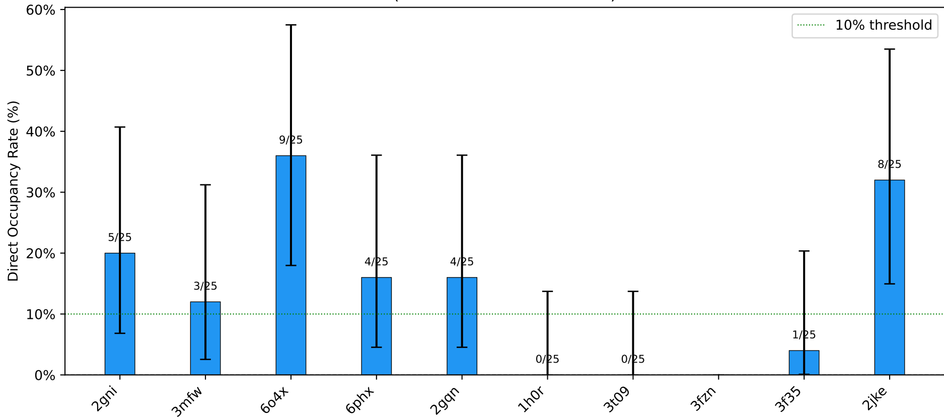
v7.1 DirectOcc Across 10 PDBbind Pockets (v6-D.2 baseline: 0% on all)
