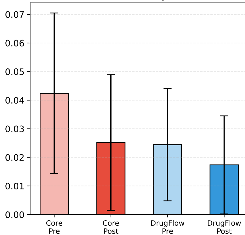
Bond Anomaly Rate
