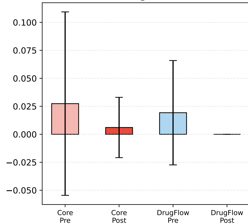
Broken Rings / Molecule
