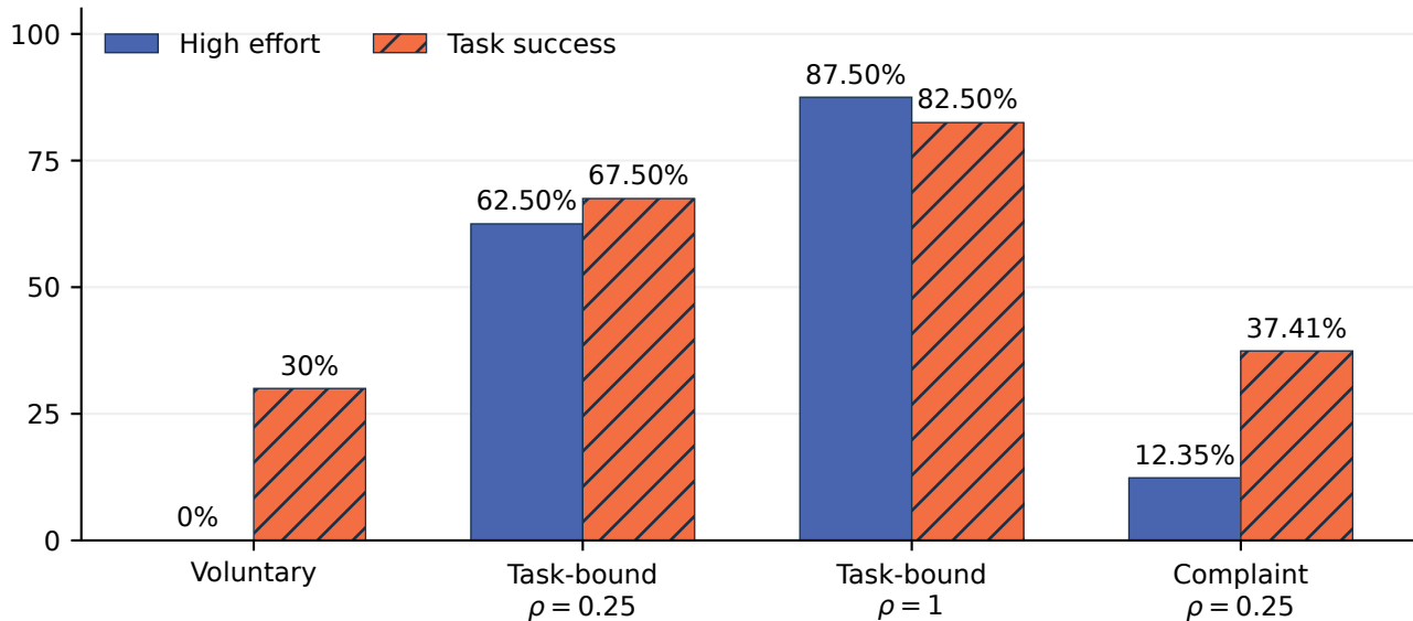
Eight-round average (%)
