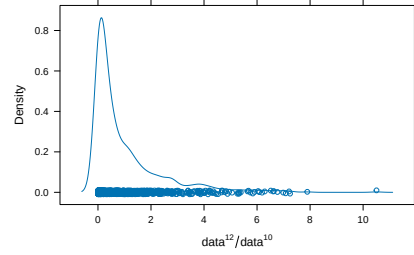
(b) Densityplot
