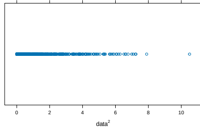
(c) Stripplot
