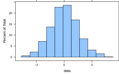
(a) Histogram
