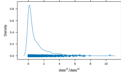
(b) Densityplot
