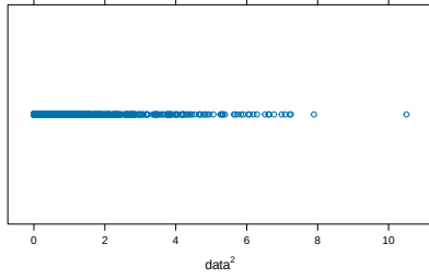
(c) Stripplot
