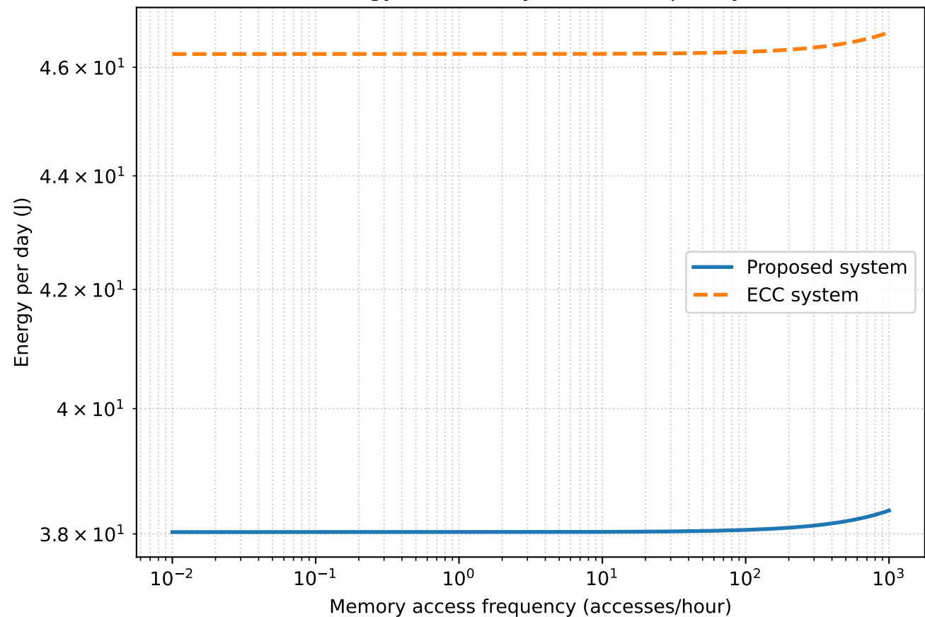
Energy vs. Memory Access Frequency
