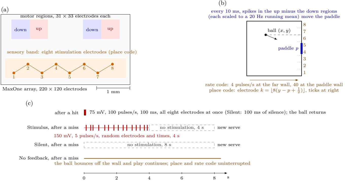
FIG. 1. DishBrain as simulated. (a) The array to scale, with the eight stimulation electrodes of the sensory band in the zig-zag of Fig. 4D of Ref. [10] and the four motor regions, counterbalanced up and down, about 1 mm away; electrode pitch 17.5 \mu\text{m} . (b) The game: the ball's height relative to the paddle selects the electrode (place code) and its distance from the paddle's wall sets the pulse rate (rate code); every 10 ms the spike counts of the up and down regions, each normalized by a running 20 Hz gain, move the paddle. (c) Feedback after each outcome in the three conditions. Rest sessions run the game with no stimulation at all. Voltages, rates, durations and the electrode layout are from Ref. [10]; court size, paddle half-length and ball speed are the model's choices (Appendix B).
