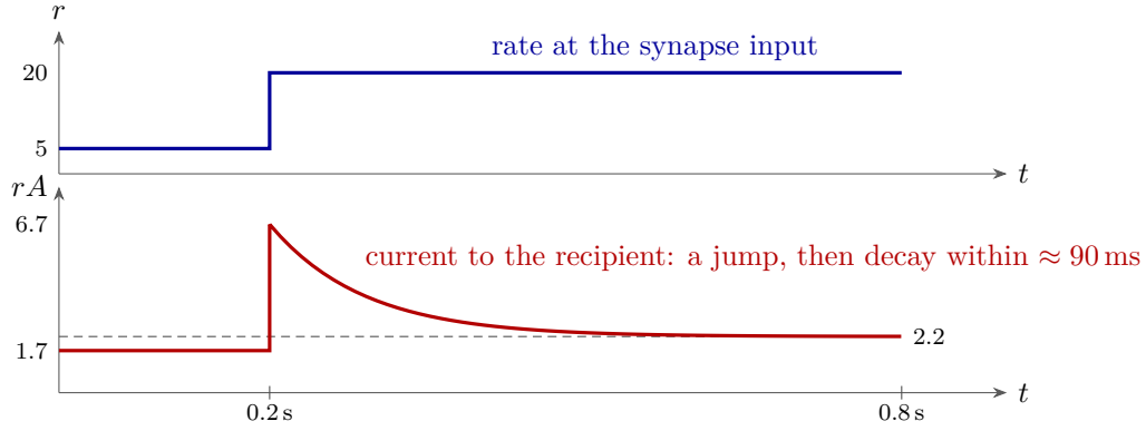
Figure 4.4: A depressing synapse according to formula (4.6) with U = 0.5 , \tau_{\text{rec}} = 0.8 s; current in units of A_0 per second; the dashed line is the steady-state current: it rose only from 1.7 to 2.2, but at the moment of the step it jumped to 6.7. The synapse tells the recipient that the rate has changed, not what it is.
