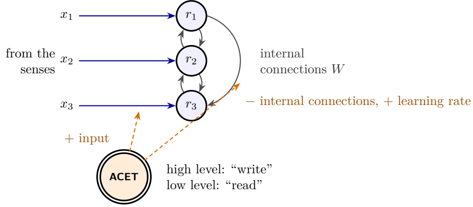
Figure 9.1: ACET as a write-enable line. Neurons r_i receive input x_i from the senses (blue arrows) and excite one another through internal connections W (gray), in which the patterns are stored. Acetylcholine (dashed arrows) strengthens the input, weakens the internal connections and makes weight changes easier, as in (9.1).
