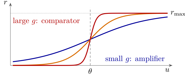
Figure 8.1: The transfer function (8.1) for three values of the gain g .
