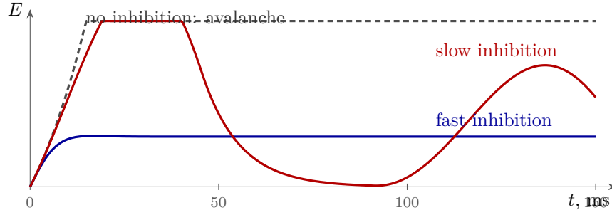
Figure 3.4: Rate of a GLUT group with feedback w_{EE} = 1.5 , \tau_E = 10 ms, after the input is switched on. Without inhibition (dashed) activity grows without bound. With inhibition of strength w_{EI}w_{IE} = 2 and \tau_I = 2 ms (blue curve) it settles at E^* = h/(1 - 1.5 + 2) = 0.67h . With the same inhibition but slow, \tau_I = 30 ms (red curve), activity oscillates.
