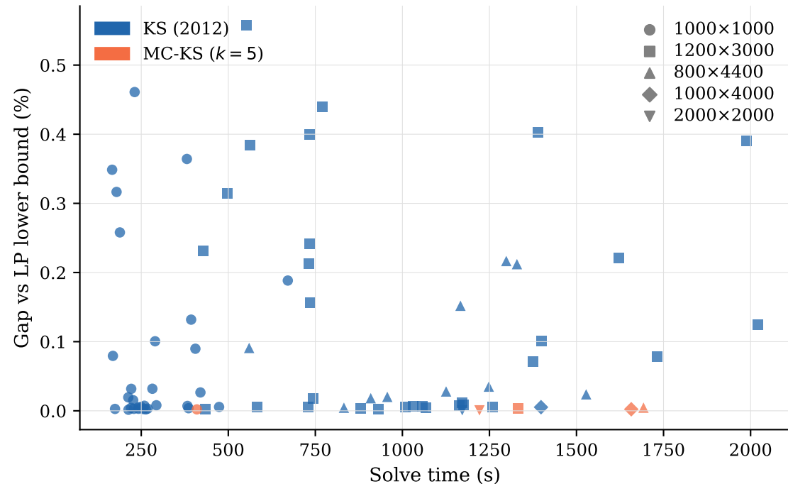
Solution quality: KS (2012) vs MC-KS — Test Bed A
