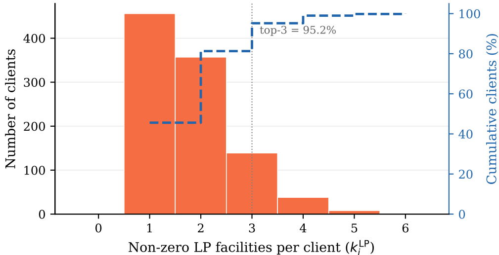
LP concentration — p1000-1000-1 (avg k_i^{\text{LP}} = 1.79 )
