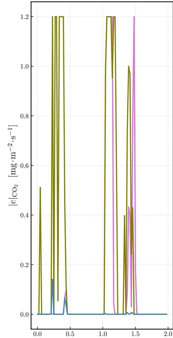
CO 2 supply rate
