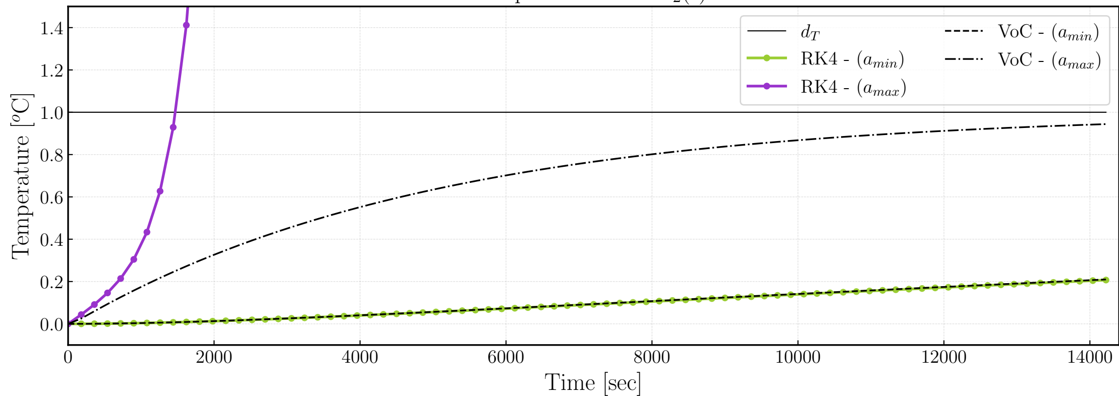
Response of State x_2(t)
