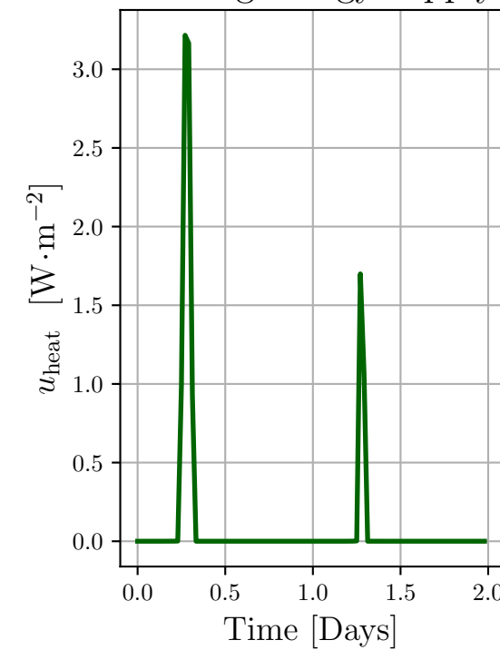
Heating energy supply
