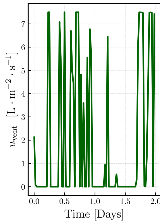
Ventilation rate
