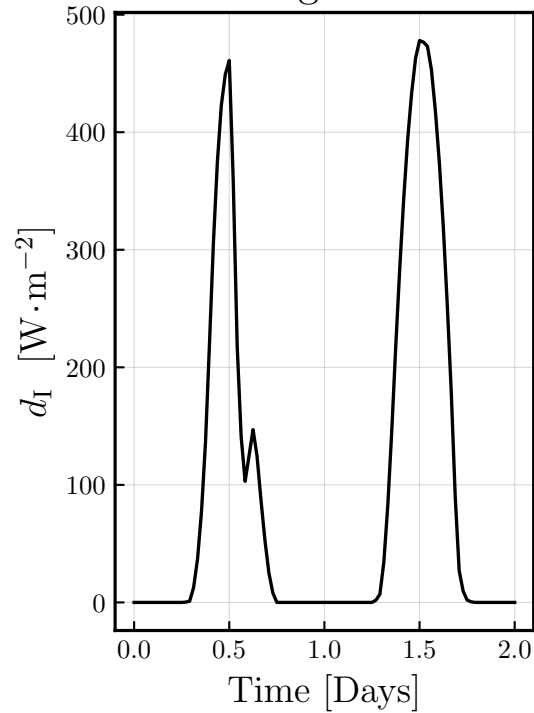
Incoming radiation
