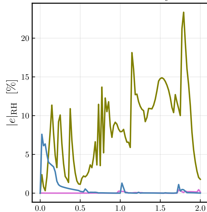
Relative Humidity
