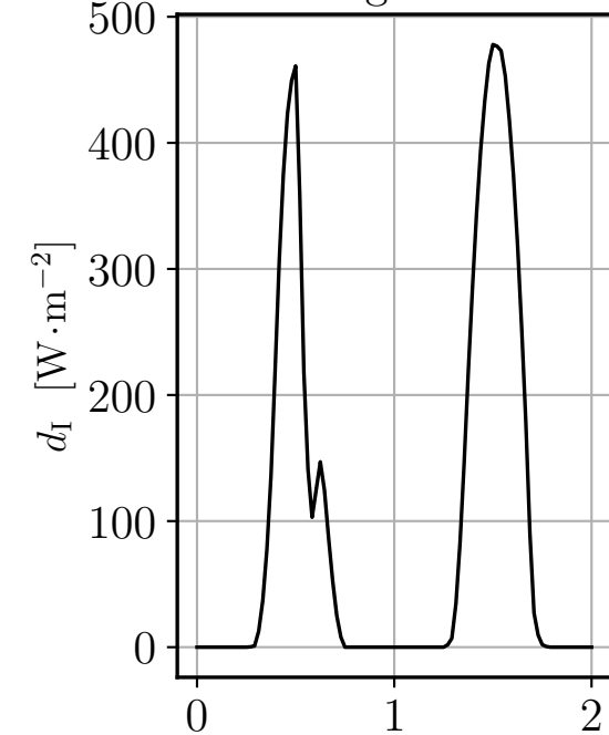
Incoming radiation
