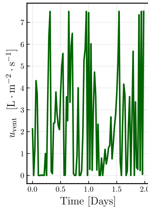
Ventilation rate
