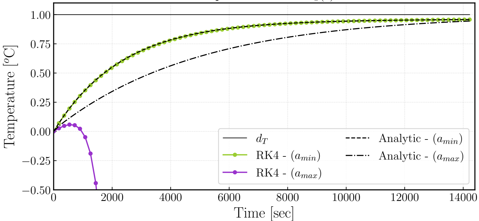
Response of State x_1(t)
