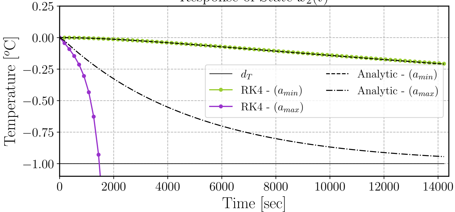
Response of State x_2(t)
