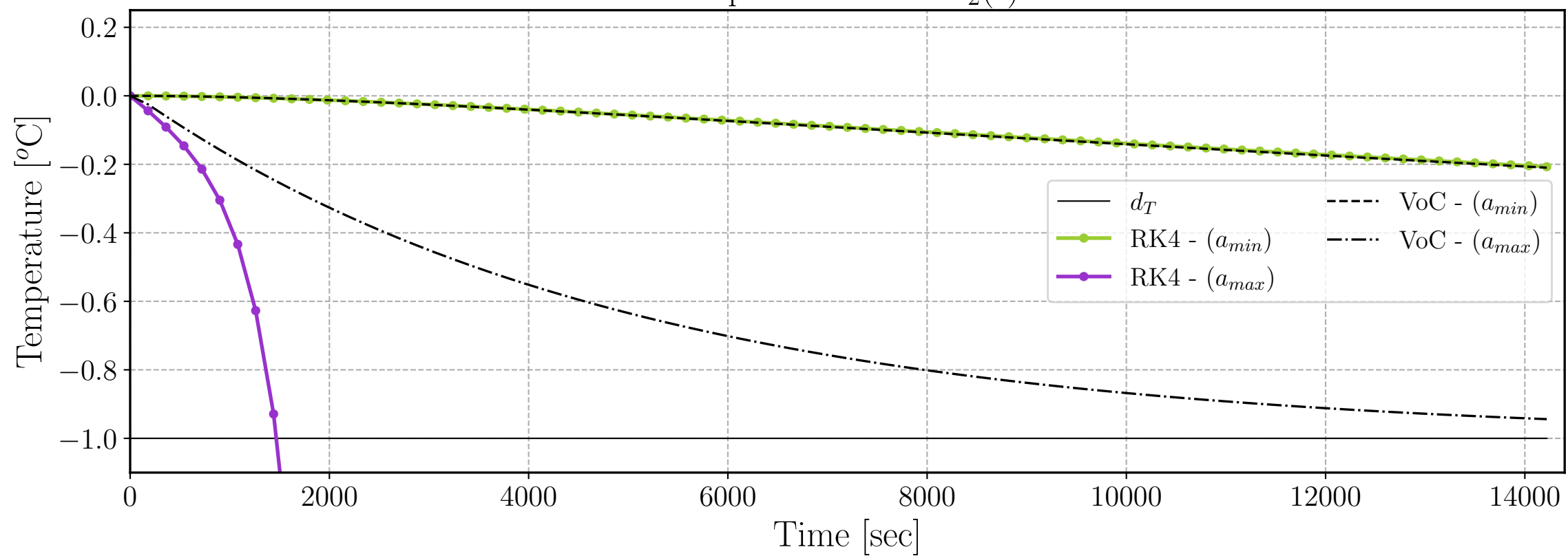
Response of State x_2(t)
