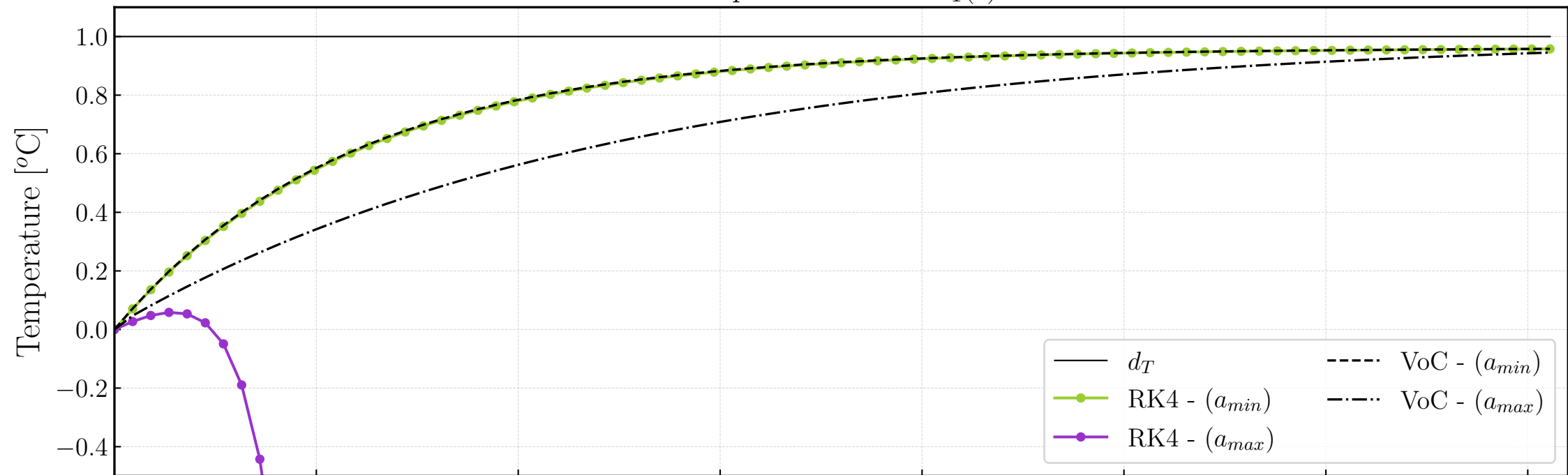
Response of State x_1(t)
