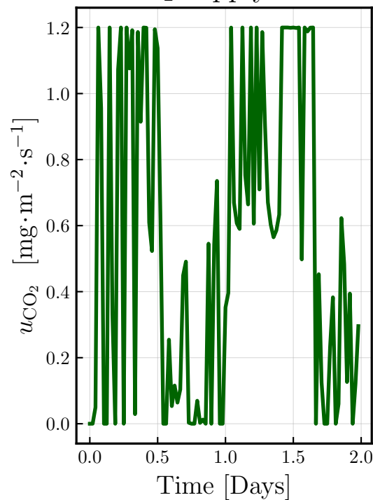
CO 2 supply rate
