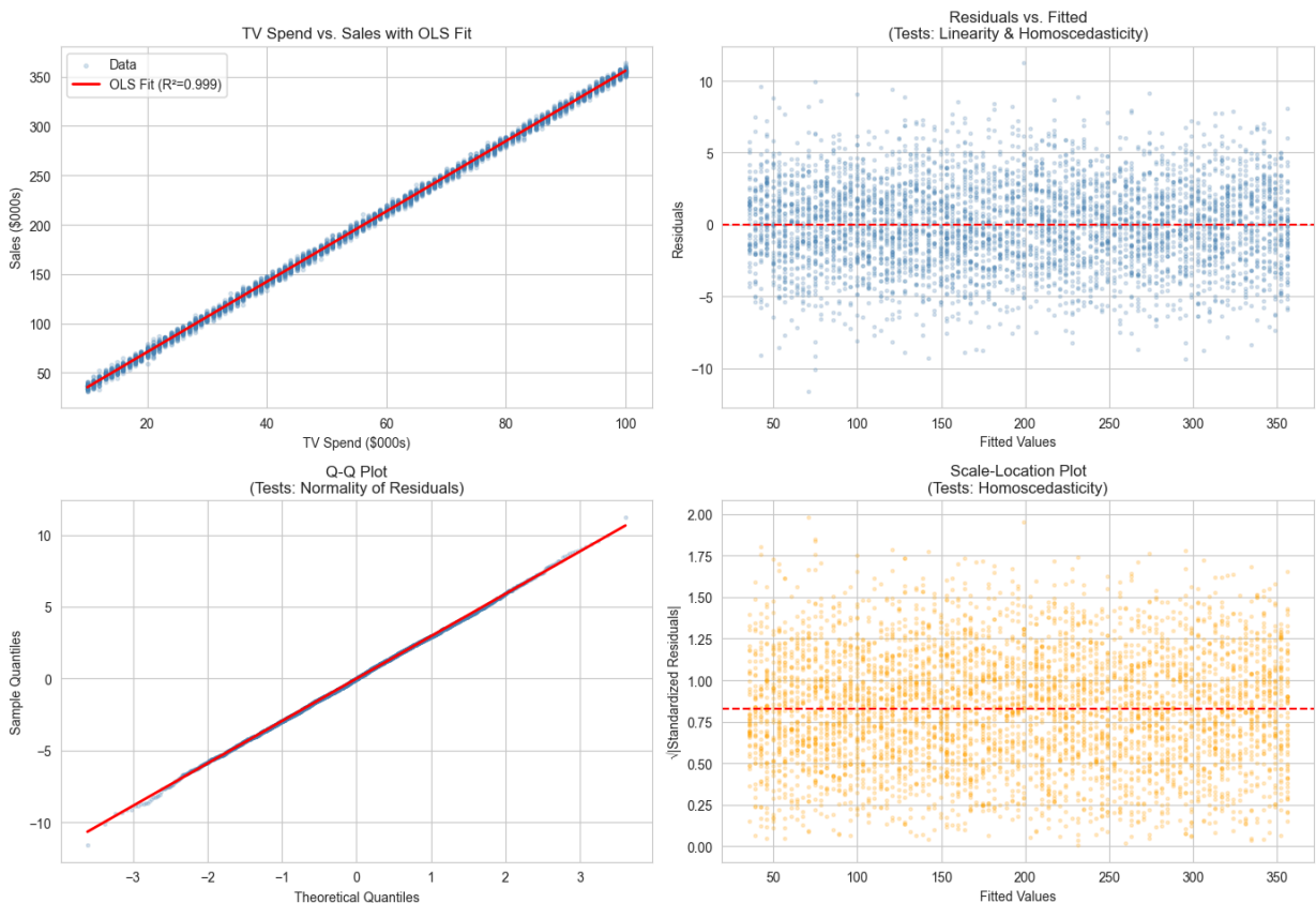
OLS Regression Diagnostic Plots
