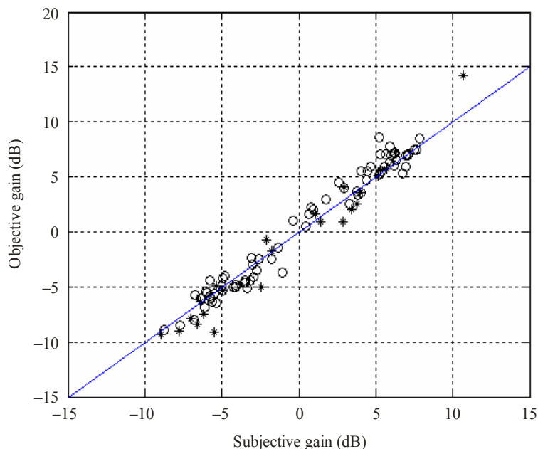
Monophonic Leq (RLB) loudness meter versus subjective results ( r = 0.982 )
