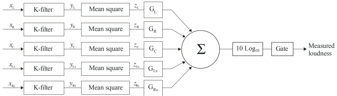
Simplified block diagram of multichannel loudness algorithm
