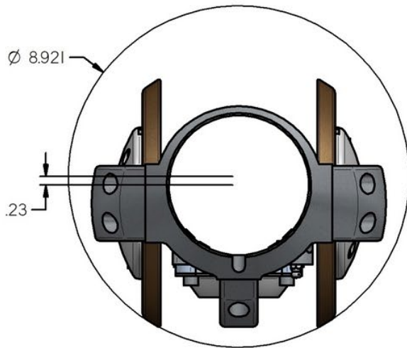
Casing OD 9-5/8" 36ppf
