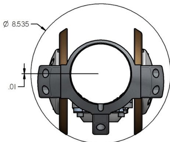
Casing OD 9-5/8" 53.5ppf
