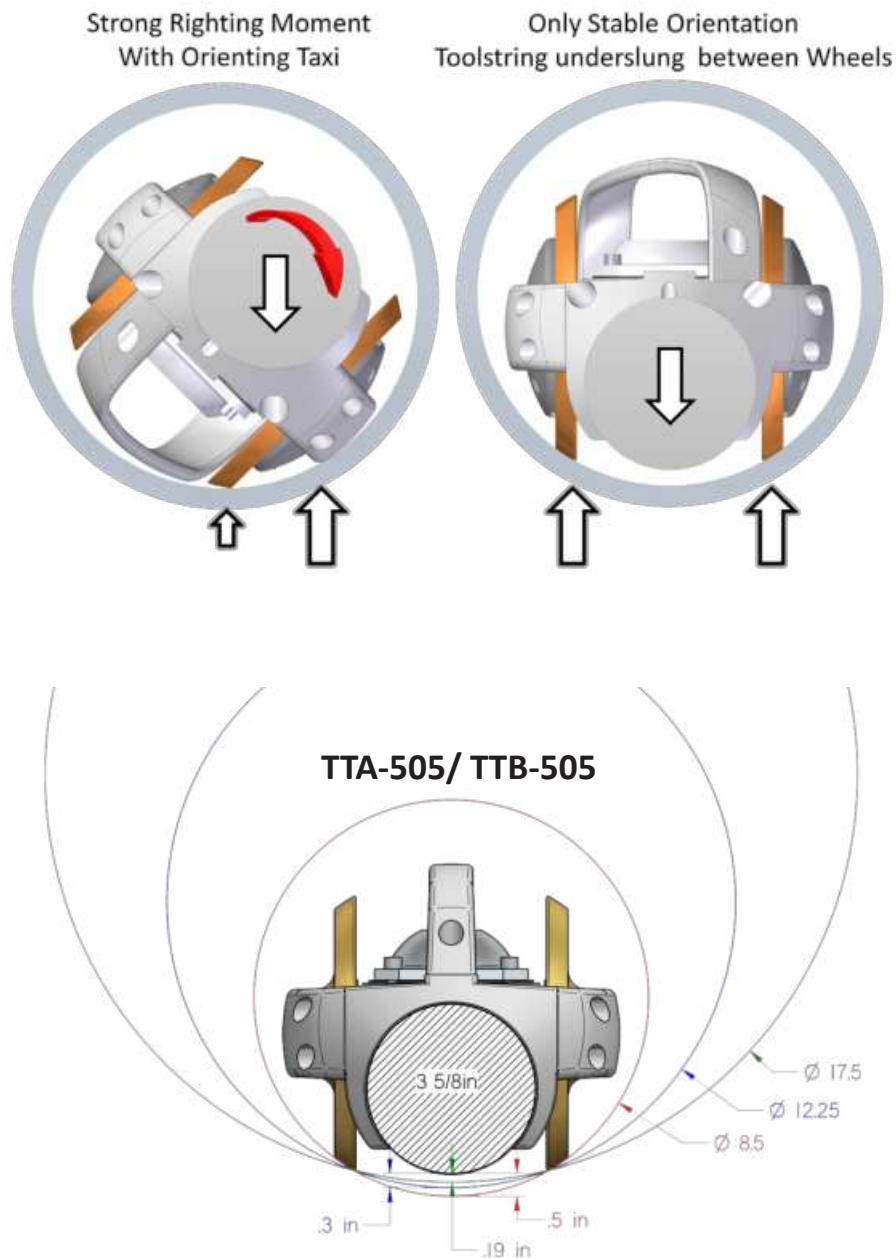
Figure 1: Standoff on a 3-5/8" Tool
