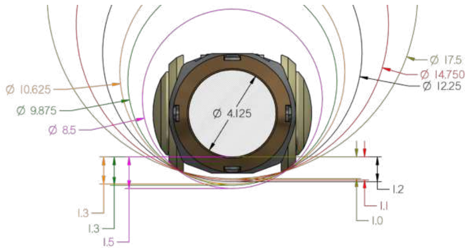
Figure: TTB - J75 Standoff for a 4-3/4" Tool
