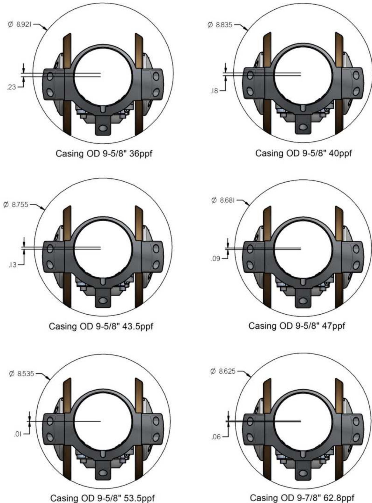
Figure 4: TTB - X515 eccentralization examples
