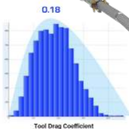
Fig.2. Actual tool drag coefficient observed during the job
