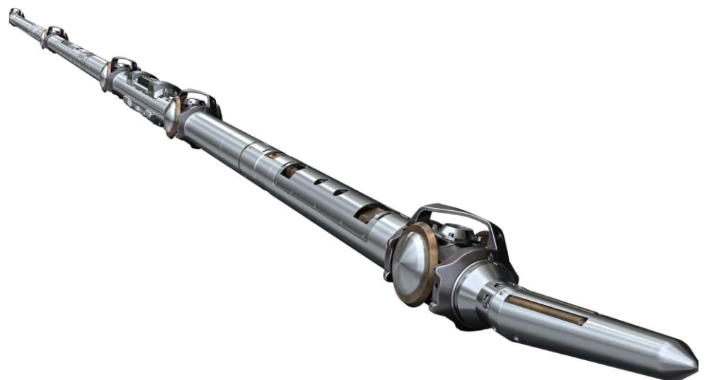
Fig1. Formation Testing Toolstring on Taxis
