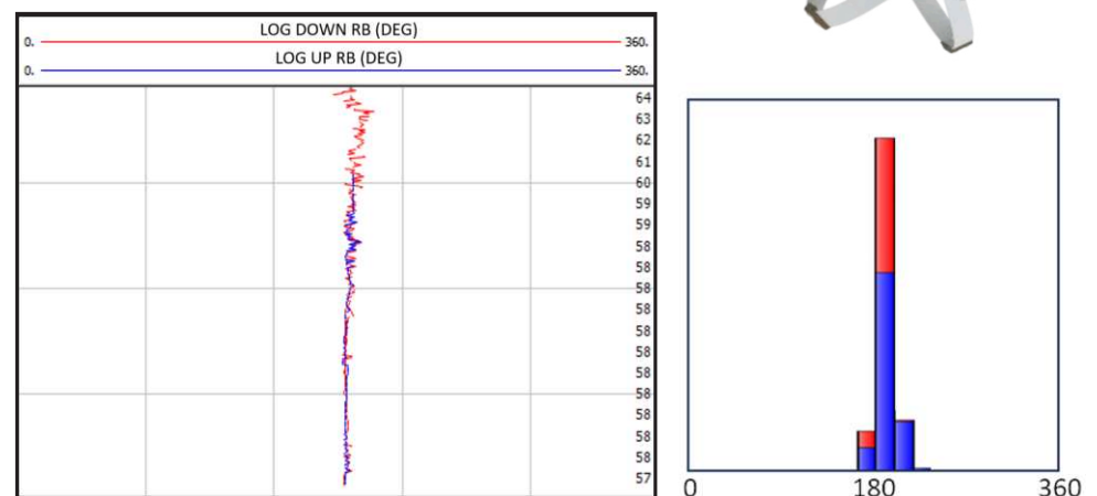
Fig 2 & 3: Log and Relative bearing Histogram showing tool on wheels
