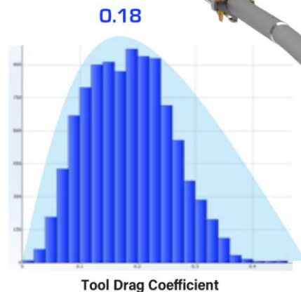
Fig.2. Actual tool drag coefficient observed during the job
