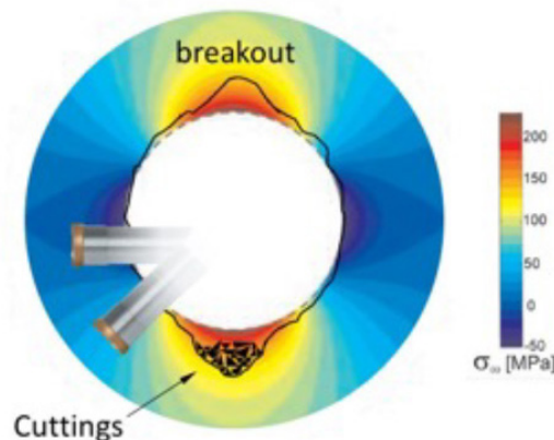
Fig.1. Cutting at 90deg to the low side of the wellbore avoids cuttings and near wellbore damage (above).
