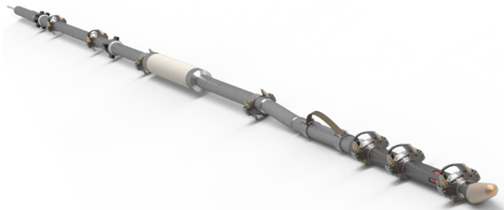
Fig.2. Petromac Wireline Express perfectly positions the MRIL-D tool in the center of the 9 5/8" casing, which maximizes the distance between the magnet and the casing. This reduces the magnetic drag to a minimum, which extends the deviation limit that the tool can be conveyed to.
