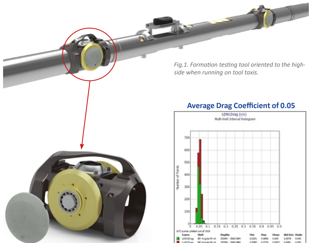
Fig.2. Average tool drag coefficient from the job – Possible to descend to 80 deg on gravity
