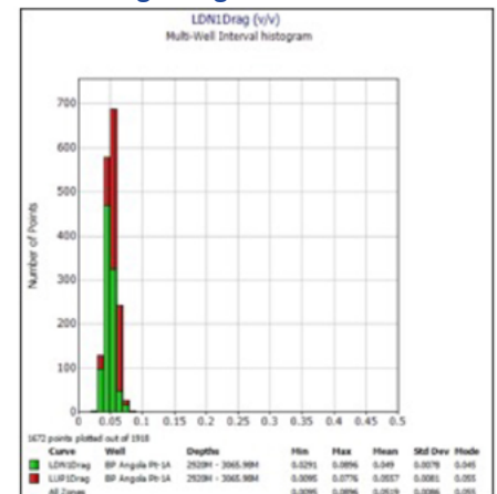
Fig.2. Average tool drag coefficient from the job – Possible to descend to 80 deg on gravity
