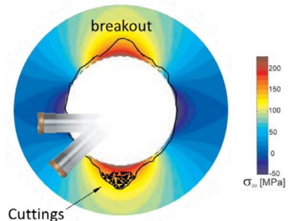
Fig.1. Cutting at 90deg to the low side of the wellbore avoids cuttings and near wellbore damage.
