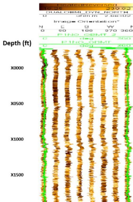
Fig.1. A single pass with dual OBMI in 12.25" hole yielded an excellent log, with no image rotation or stick slip.
