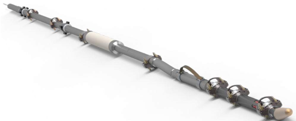
Fig.2. Petromac Wireline Express perfectly positions the MRIL-D tool in the center of the 9 5/8" casing, which maximizes the distance between the magnet and the casing. This reduces the magnetic drag to a minimum, which extends the deviation limit that the tool can be conveyed to.
