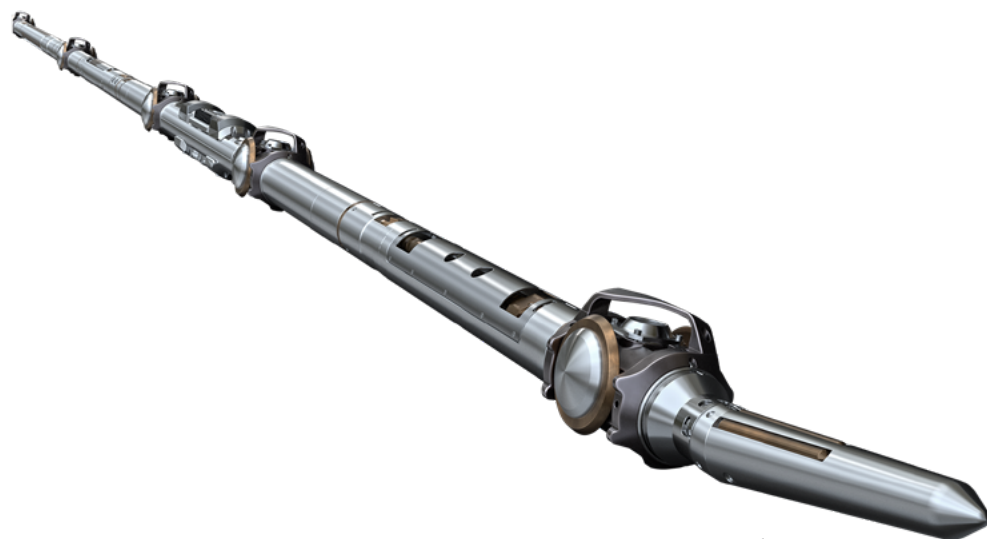
Fig1. Formation Testing Toolstring on Taxis
