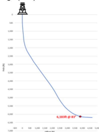
Fig 3: Well 6 trajectory
