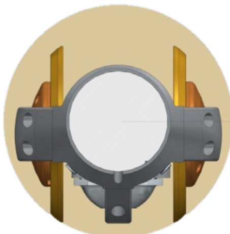
Fig.1. Centralizing Tool Taxis provide 2.4" of standoff, which keep the Array Sonic within .1" of the center of the wellbore in 8.5" hole.
