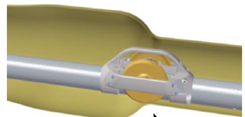
Tool Taxi wheels roll over ledge
