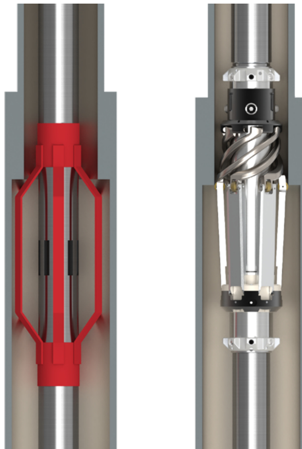
Fig 1: Conventional centralisers are designed to centralize in only one casing size at a time. Helix passes through any restrictions seamlessly and centralizes in multiple casing sizes.
