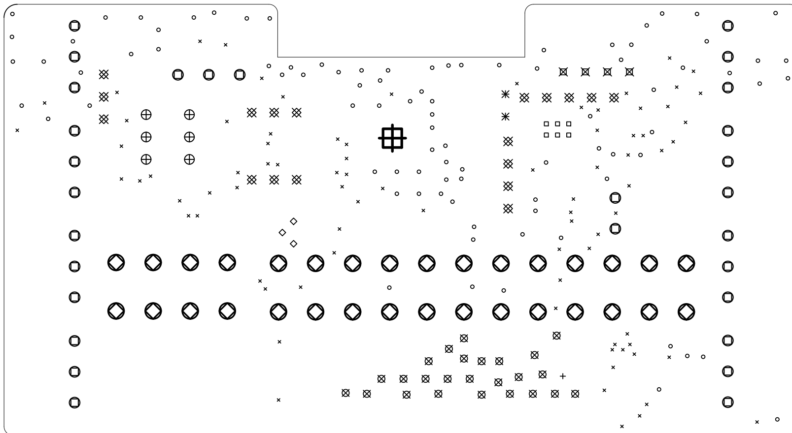
Drill Map:
