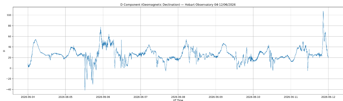
Figure 6: Hobart Geomagnetic Observatory geomagnetic declination data 04-12/06/2026. UT time. (Space Weather Services (Bureau of Meteorology), World Data Centre for Geomagnetism).
