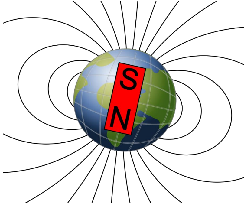
Figure 1: Earth's magnetic field lines form closed loops around the planet. Magnetic north is in the southern hemisphere, and magnetic south is in the northern hemisphere. (Zureks, CC0 1.0 , via Wikimedia Commons )
