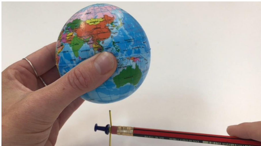
Figure 3: Paperclip is perpendicular to Earth's surface at the poles.
