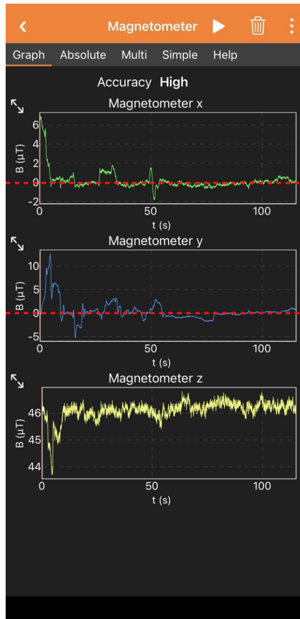
Figure B: Labelled screenshot of the phyphox magnetometer in Graph mode with B_x and B_y brought to 0. The red dashed lines mark the location of 0 \mu T for reference (phyphox app (RWTH Aachen University), used under CC BY 4.0 ).
