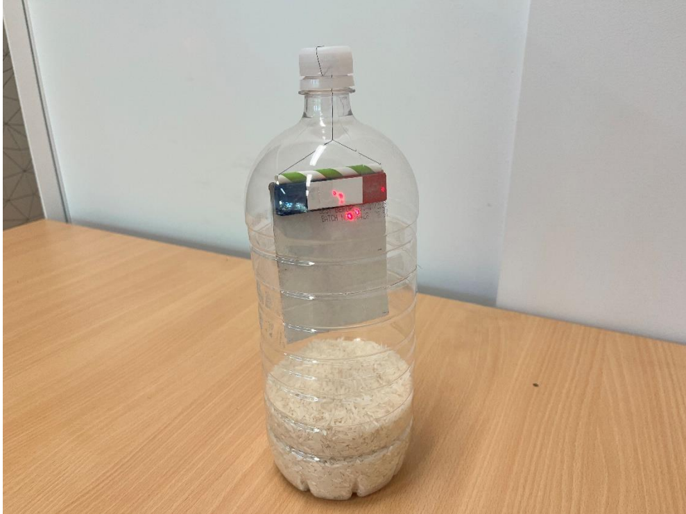
Figure 7: Laser pointer hits the centre of the mirror card on the magnet.
