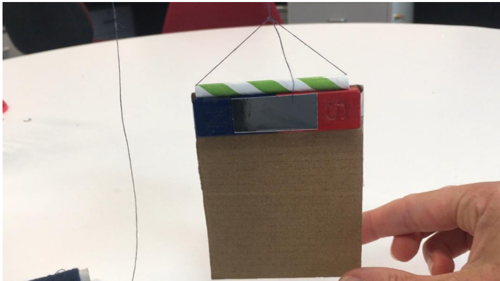
Figure 3: Bar magnet with the straw stuck to the top and mirror card stuck to the centre. These are taped to a piece of cardboard ~10cm long. Cotton thread is threaded through the straw and tied as a triangular loop with sides of equal length (a few cm).
