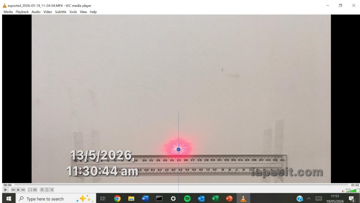
Figure 11: A frame from a pop bottle magnetometer timelapse with a blue shape added to the centre of the laser spot in Microsoft PowerPoint to make tracking changes in the spot position easier.
