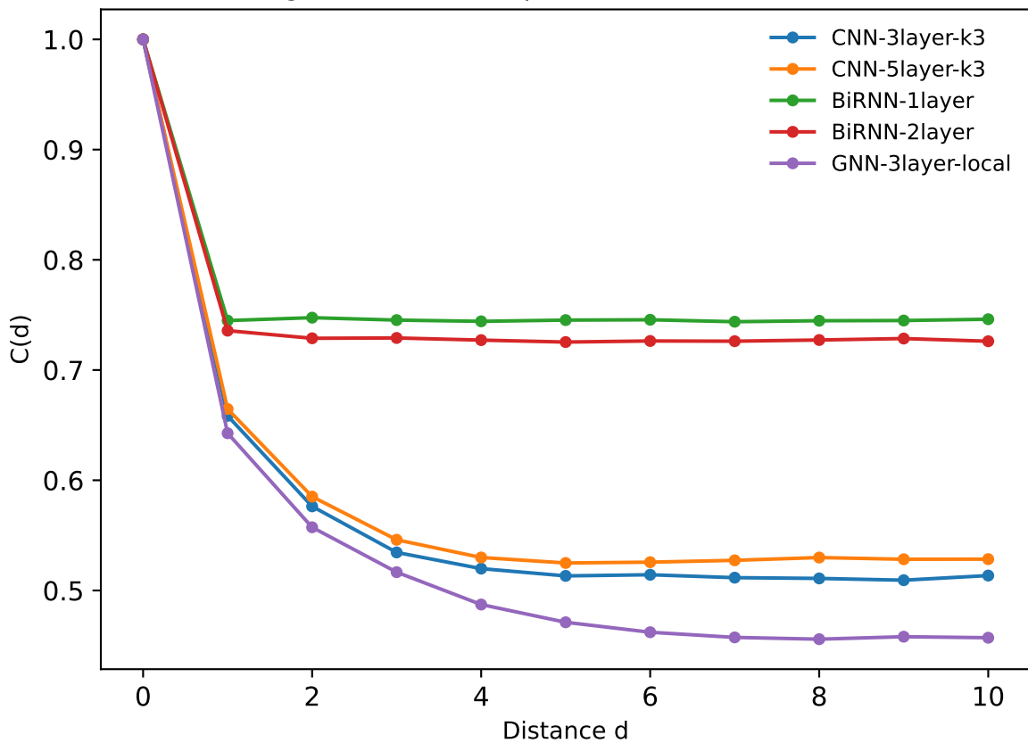
Fig 8 - Learned two-point correlation functions
