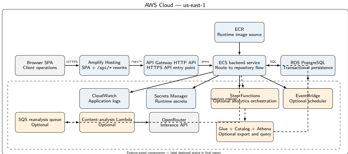
Figure 2: Deployment and component overview. The primary path is the active topology documented in infrastructure source; content analysis and analytics are feature-gated and must be status-labelled in the final report.
