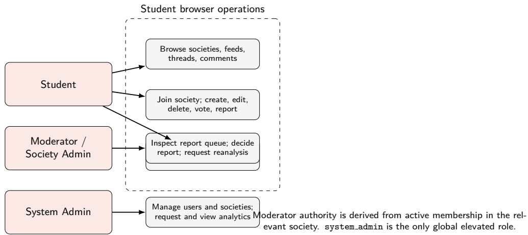
Figure 1: Product roles and client operations. The diagram orients the reader; the operation coverage table and Figures 3–6 provide the downstream invocation paths.
