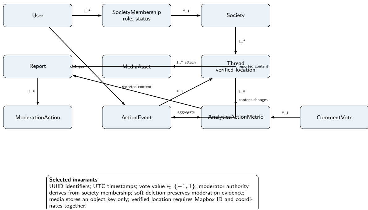
Figure 7: Simplified logical data model. It communicates relationships and invariants rather than every physical column.
