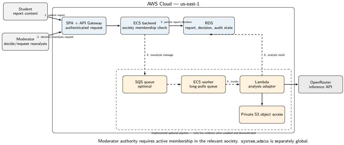
Figure 5: Moderation and optional content-analysis flow. Orange elements are feature-gated; do not claim them as deployed evidence without an end-to-end observation.
