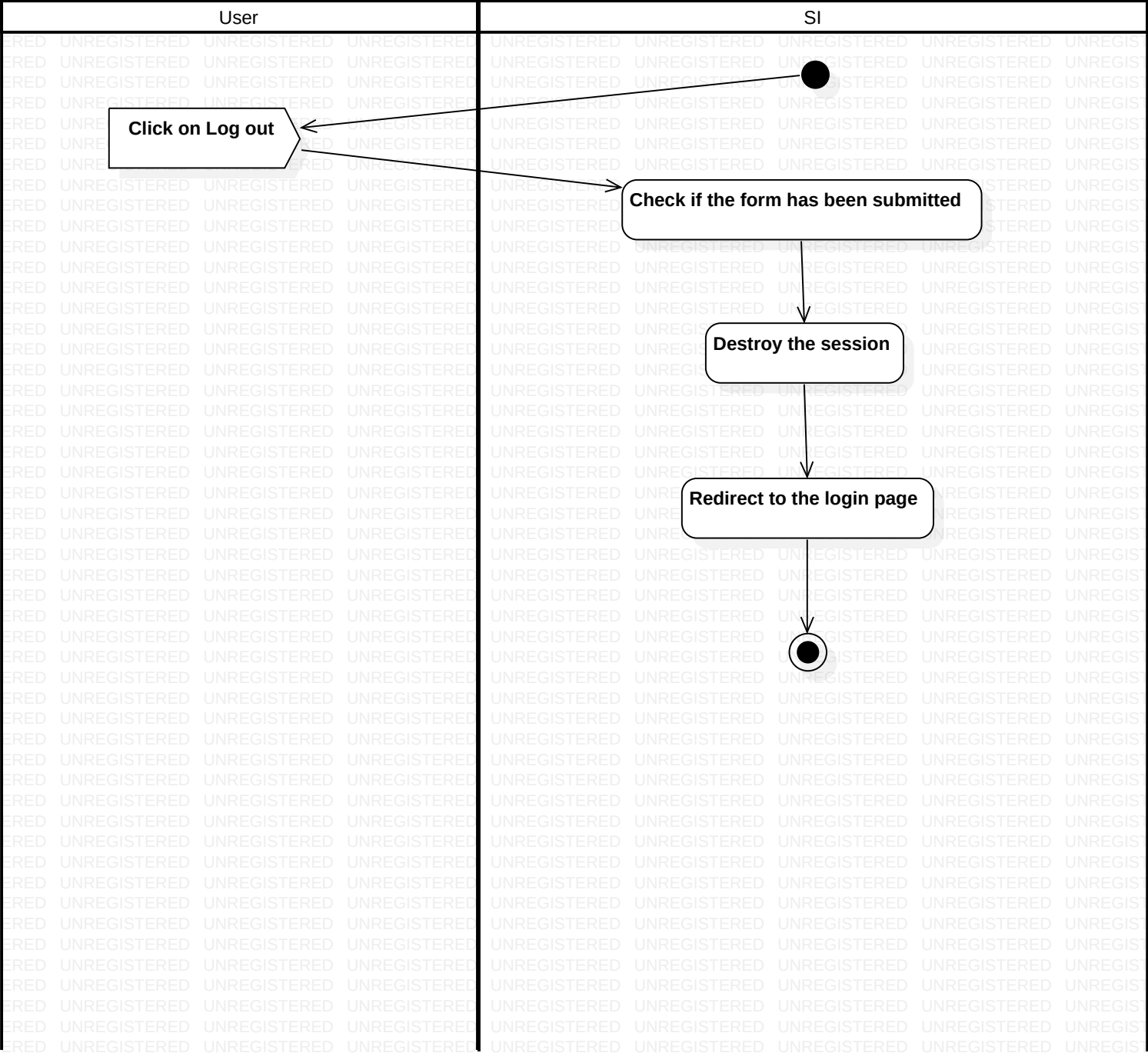
Activity1::ActivityDiagram1
