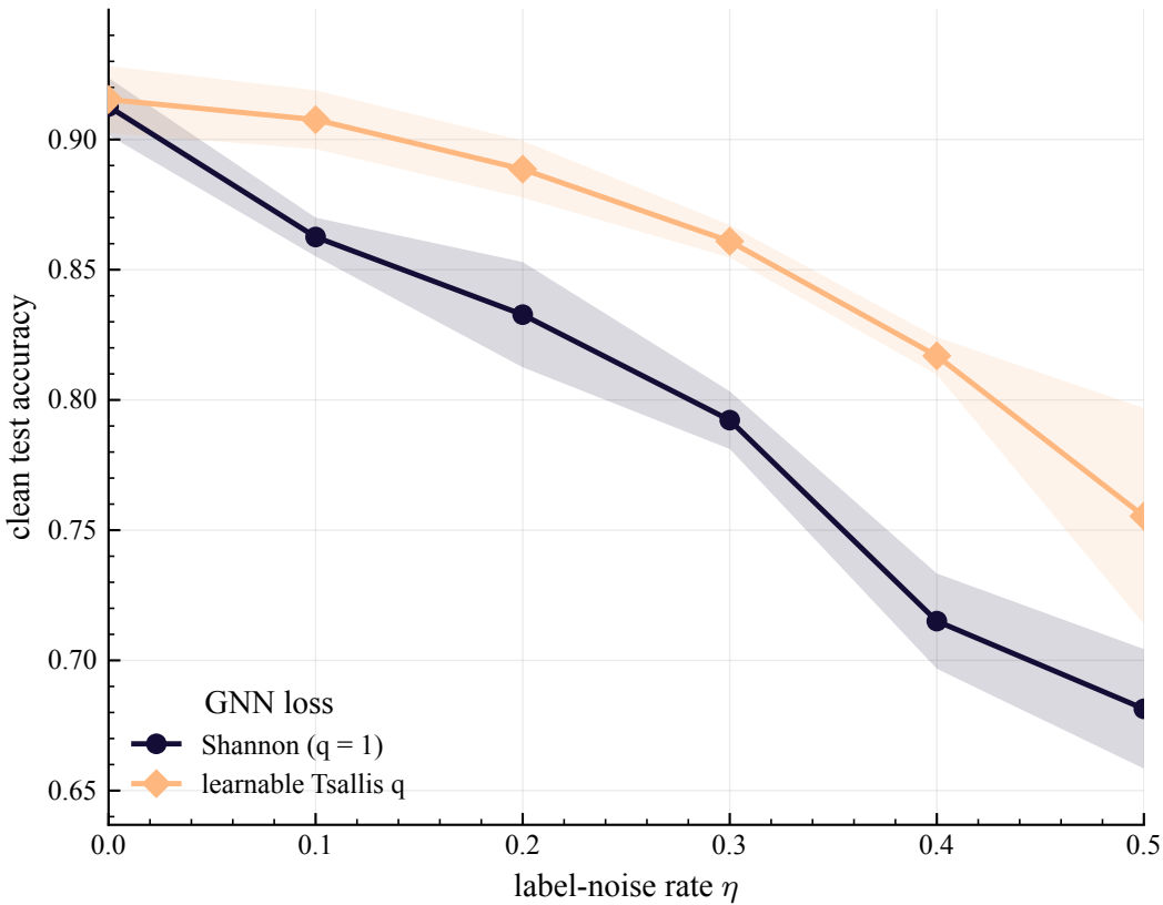
(a) robustness to label noise
