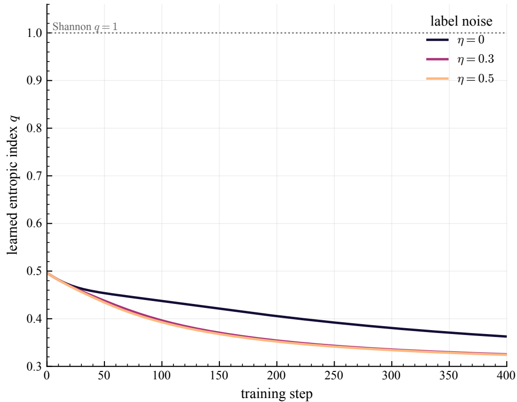
(b) q descends to the robust regime
